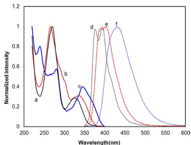
Figure 4. Normalized absorbance spectra (—) and fluorescence spectra (---) of phenanthrene compounds, TphP (black, a,d), TnaP (red, b,e), and TpyP (blue, c,f), in MeCN:Bz (v:v = 1:1). Emission spectra were excited at the absorption maximum.
