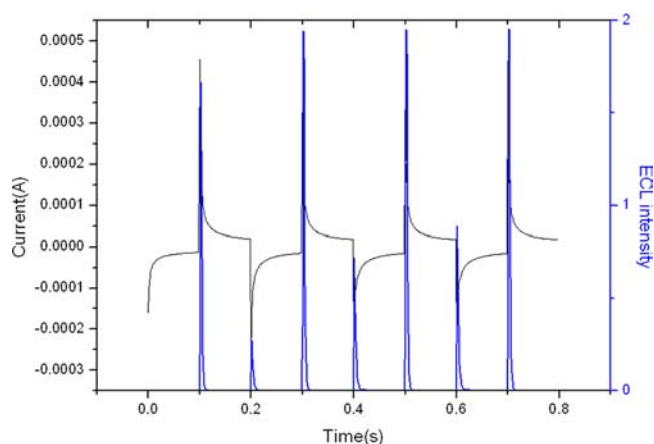
Figure 6. Initial current (black) and ECL light (blue) transients for 0.5 mM TphP pulsed between 80 mV past the first reduction peak and at 80 mV past the first oxidation potential, respectively. Pulse width is 0.1 s.
