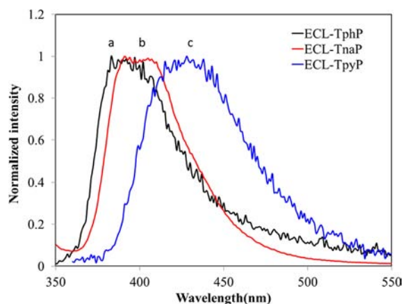
Figure 5. ECL spectra of TphP (black, a), TnaP (red, b), and TpyP (blue, c) generated through annihilation by pulsing the potential with a pulse width of 0.1 s from approximately 80 mV past the peaks potentials; slit width: 20 nm.
